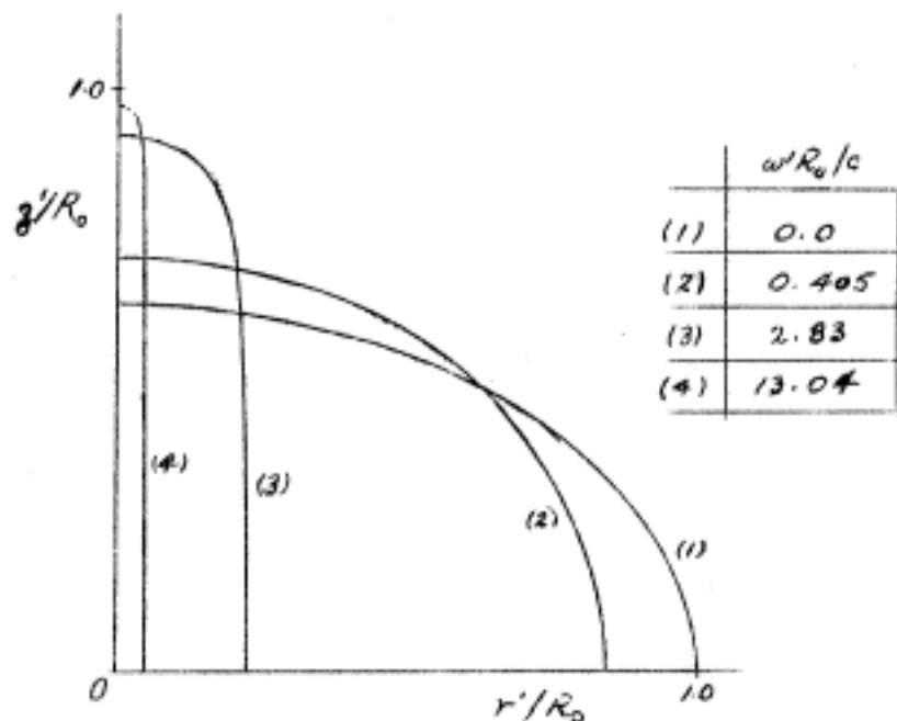
Fig. 6C: Deformation of meridian section of sphere in uniform screw motion ( \delta fixed).
