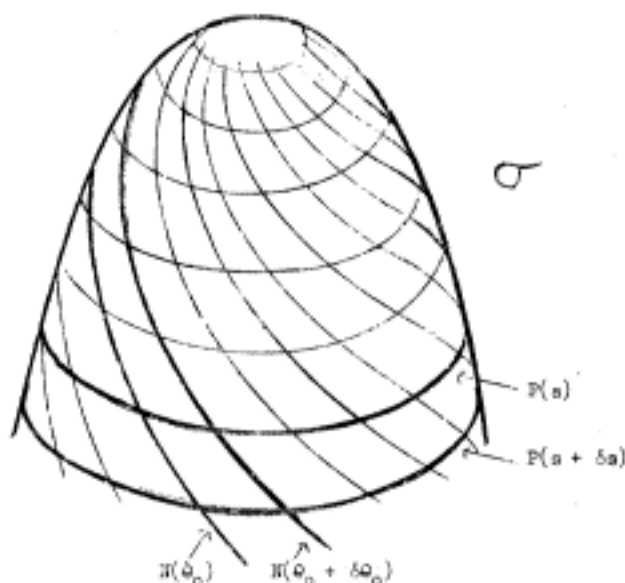
Fig. 3B: Surface of revolution in symmetrical motion
