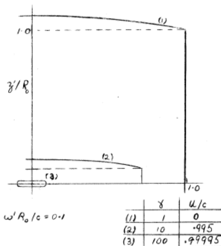
Fig. 7B: Deformation of meridian section of circular cylinder in uniform screw motion ( \omega' fixed)
