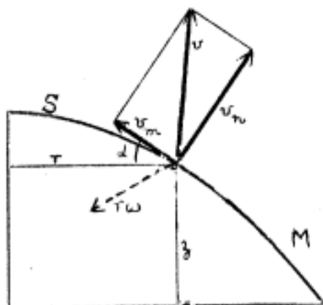
Fig. 3C: Velocity components in meridian plane
