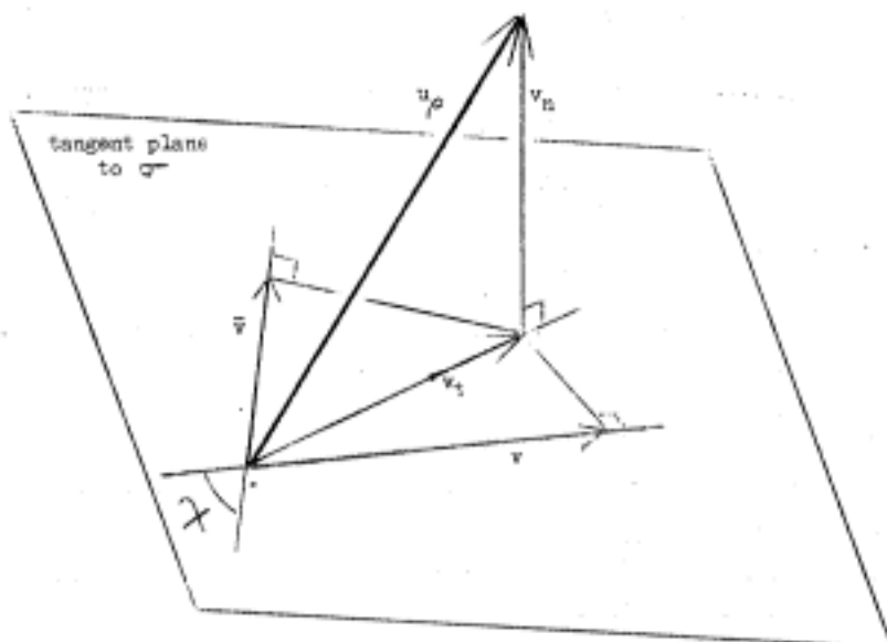
Fig. 2C: Velocity components on a surface.
