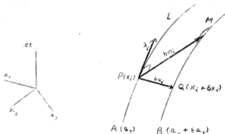
Fig. 2A: Two rigidly connected particles in space-time
