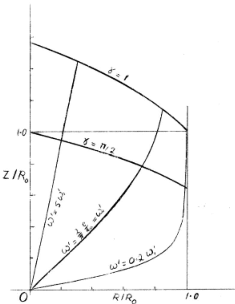
Fig. 6A: Maximum height Z and radius R of rigid sphere in uniform screw motion with speed U and spin \omega' . \delta = (1 - U^2/c^2)^{-1/2} .
