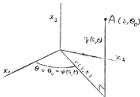
Fig. 3A1. Coordinates for surface of revolution in symmetrical motion
